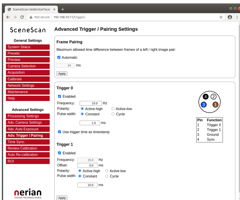
Figure 27: Screenshot of configuration page for trigger settings.
