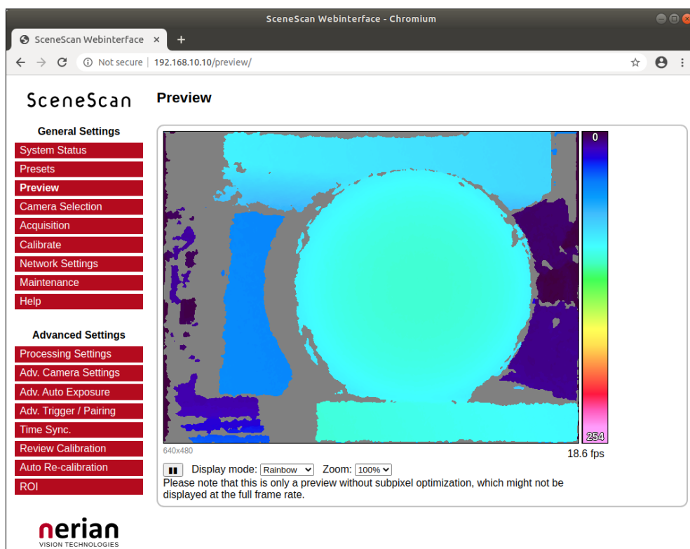
Figure 16: Screenshot of configuration preview page.
