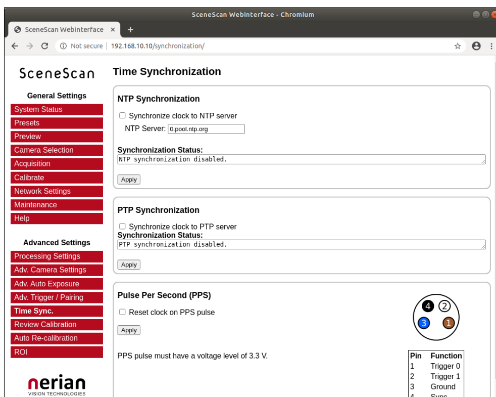
Figure 28: Screenshot of configuration page for time synchronization.
