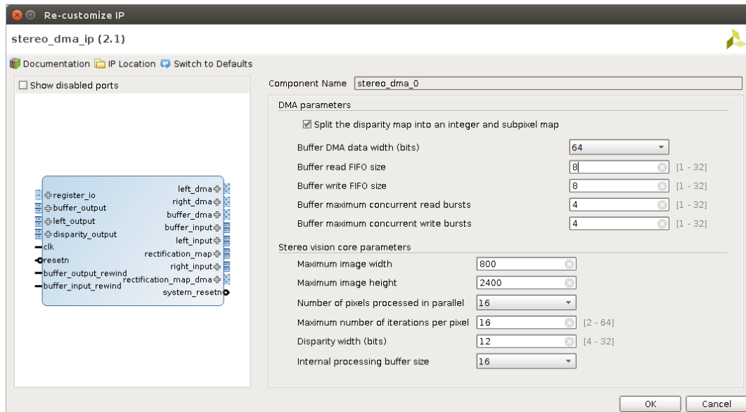
Figure 8: Configuration parameters of DMA core.
